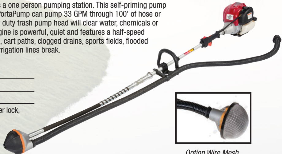
Option Wire Mesh Sand Screen (PP-L80SS)
